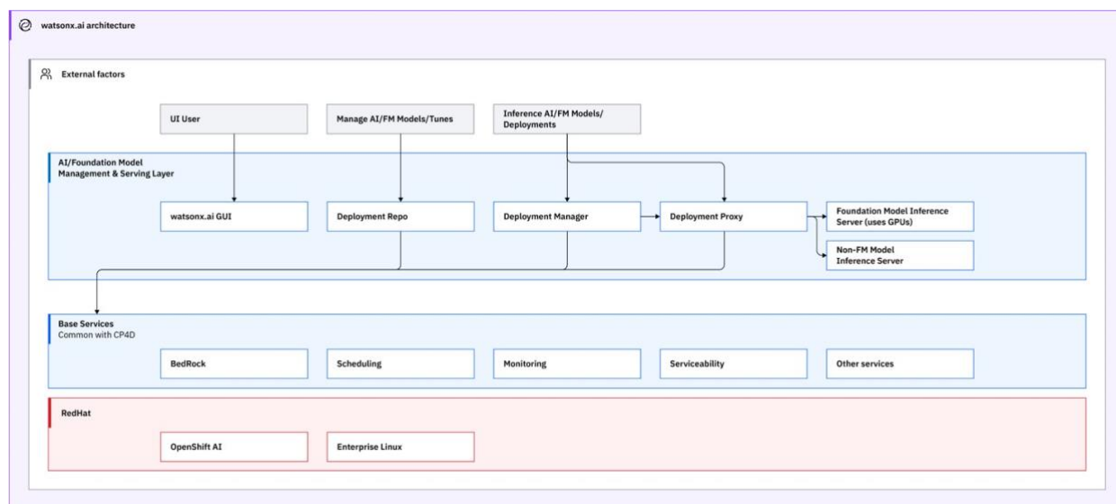
Figure 3: watsonx.ai architecture
