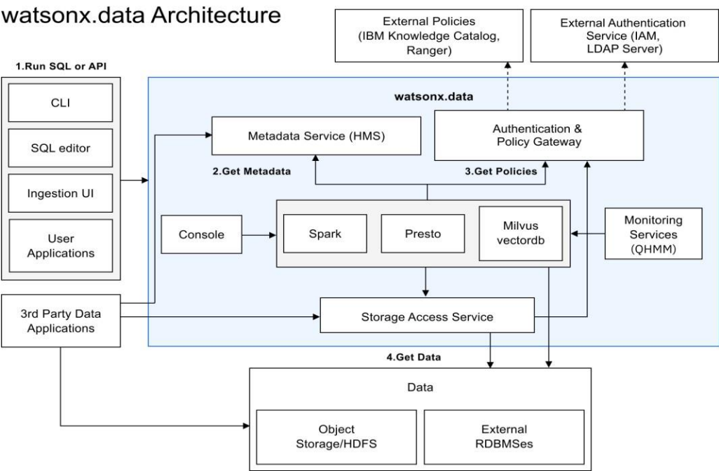
Figure 3: watsonx.data architecture
